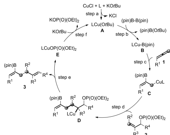
Scheme 4. A possible catalytic cycle.
